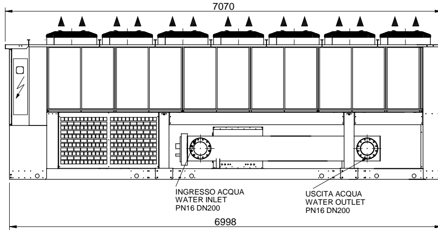
VISTA LATERALE SIDE VIEW
