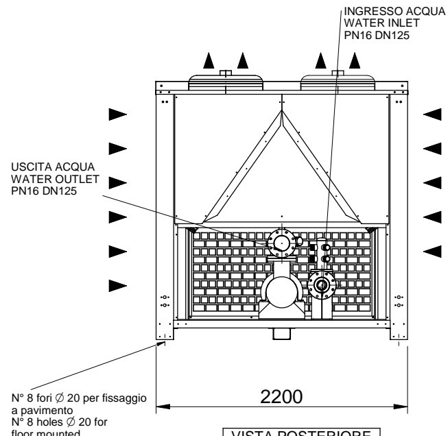
VISTA POSTERIORE BACK VIEW
