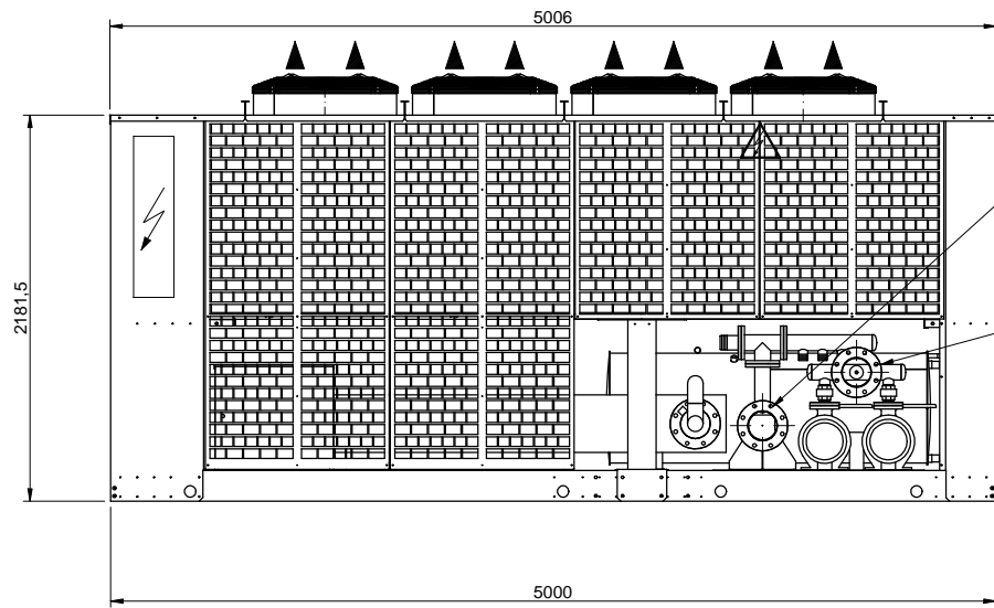
VISTA LATERALE SIDE VIEW
