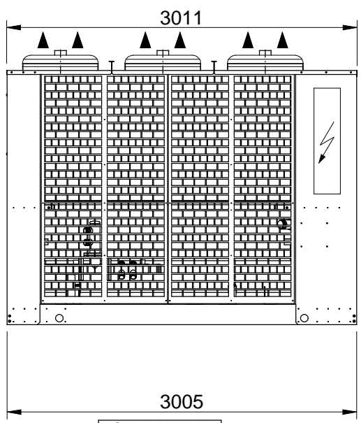
VISTA LATERALE SIDE VIEW
