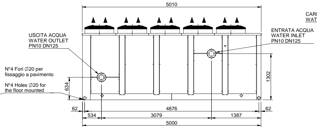
VISTA LATERALE SIDE VIEW
