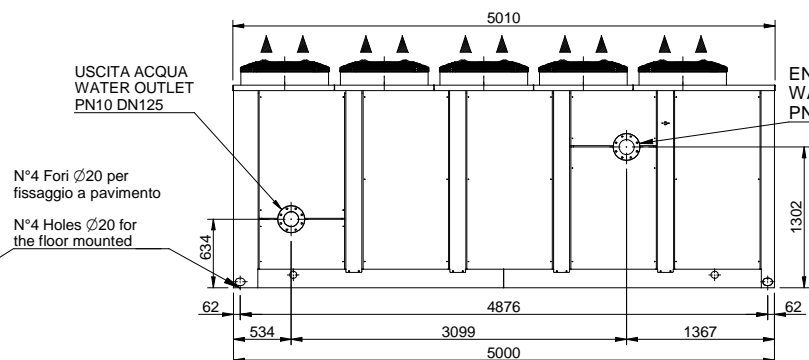
VISTA LATERALE SIDE VIEW
