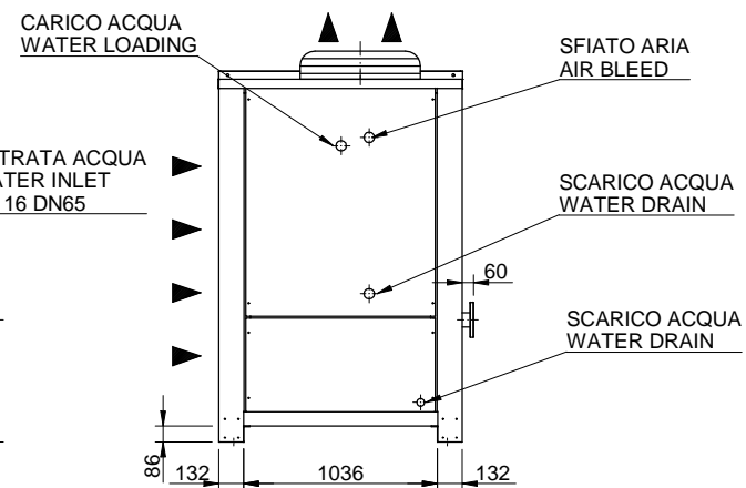
VISTA POSTERIORE BACK VIEW
