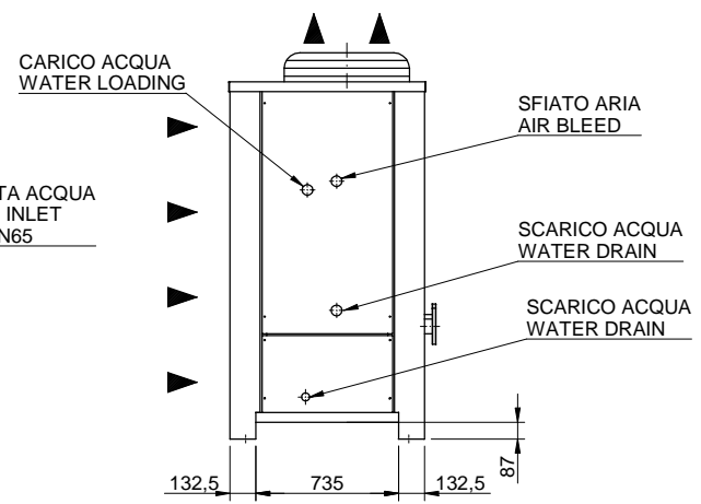
VISTA POSTERIORE BACK VIEW
