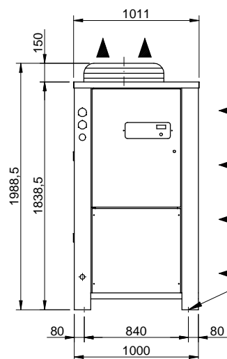
VISTA FRONTALE FRONT VIEW
