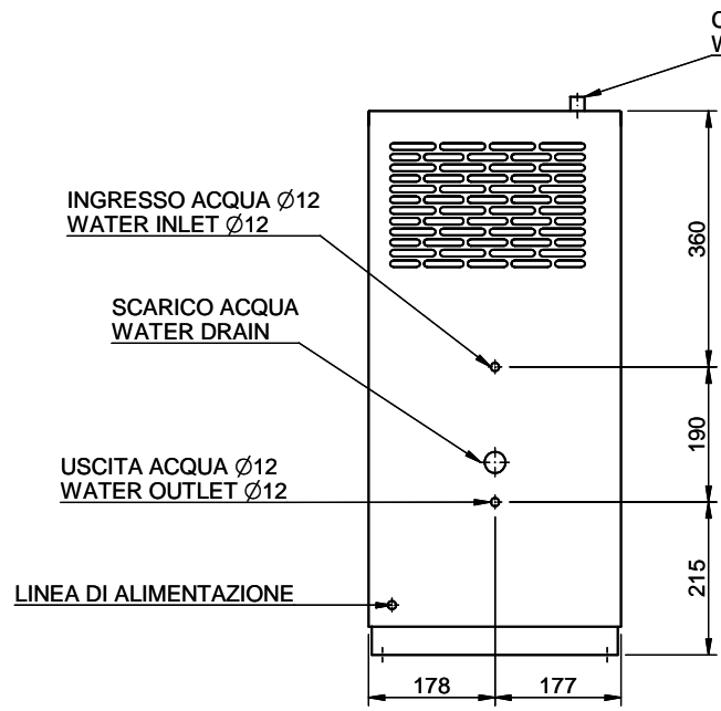
VISTA POSTERIORE BACK VIEW
