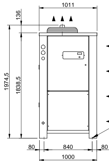
VISTA FRONTALE FRONT VIEW
