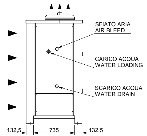
VISTA POSTERIORE BACK VIEW
