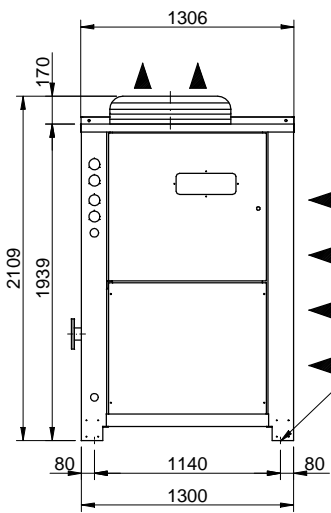
VISTA FRONTALE FRONT VIEW
