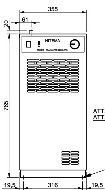
VISTA FRONTALE FRONT VIEW
