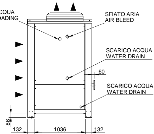
VISTA POSTERIORE BACK VIEW
