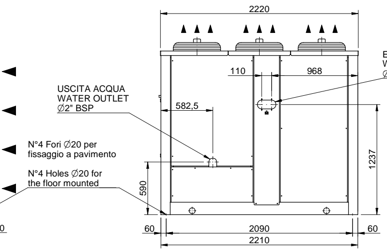
VISTA LATERALE SIDE VIEW
