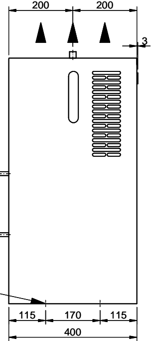
VISTA LATERALE SIDE VIEW
